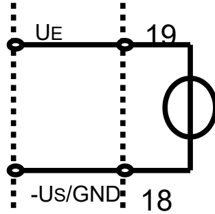
Drawing 3: 37-pole Sub-D socket, CH 3
