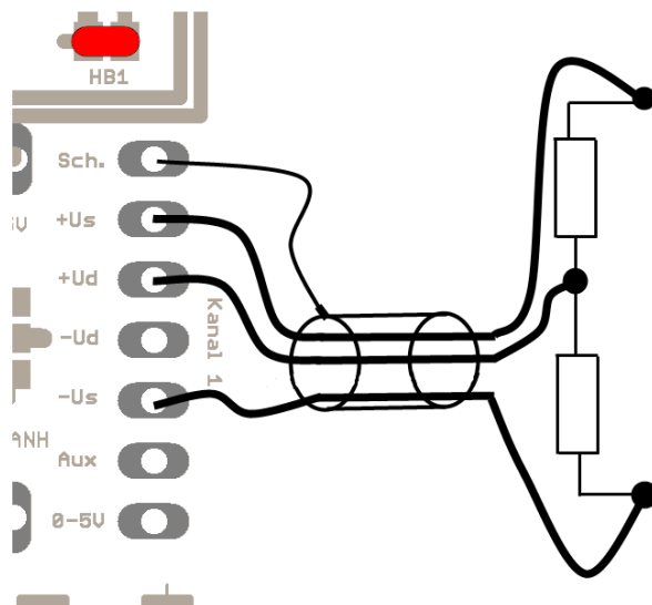
Figure 7: Straingage-Half bridge
