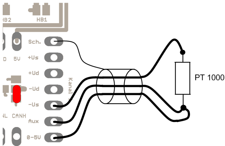
Figure 9: PT1000
