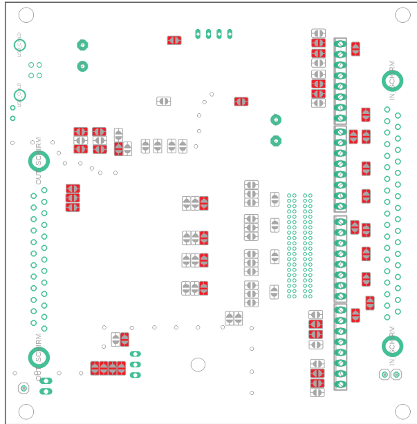
Figure 1: M12_standard variant
