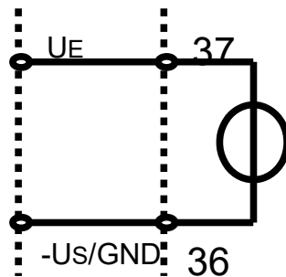
Drawing 5: 37-pole Sub-D socket, CH 4
