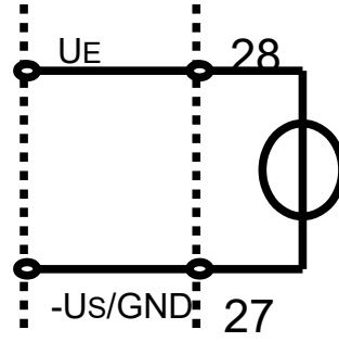
Drawing 2: 37-pole Sub-D socket, CH 1
