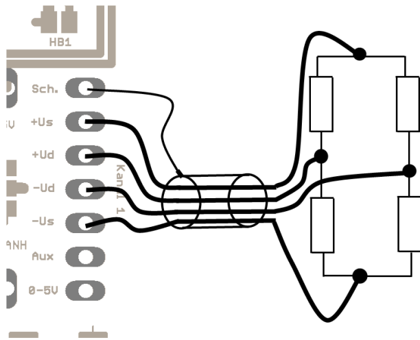
Figure 8: Strain gauge-Full bridge
